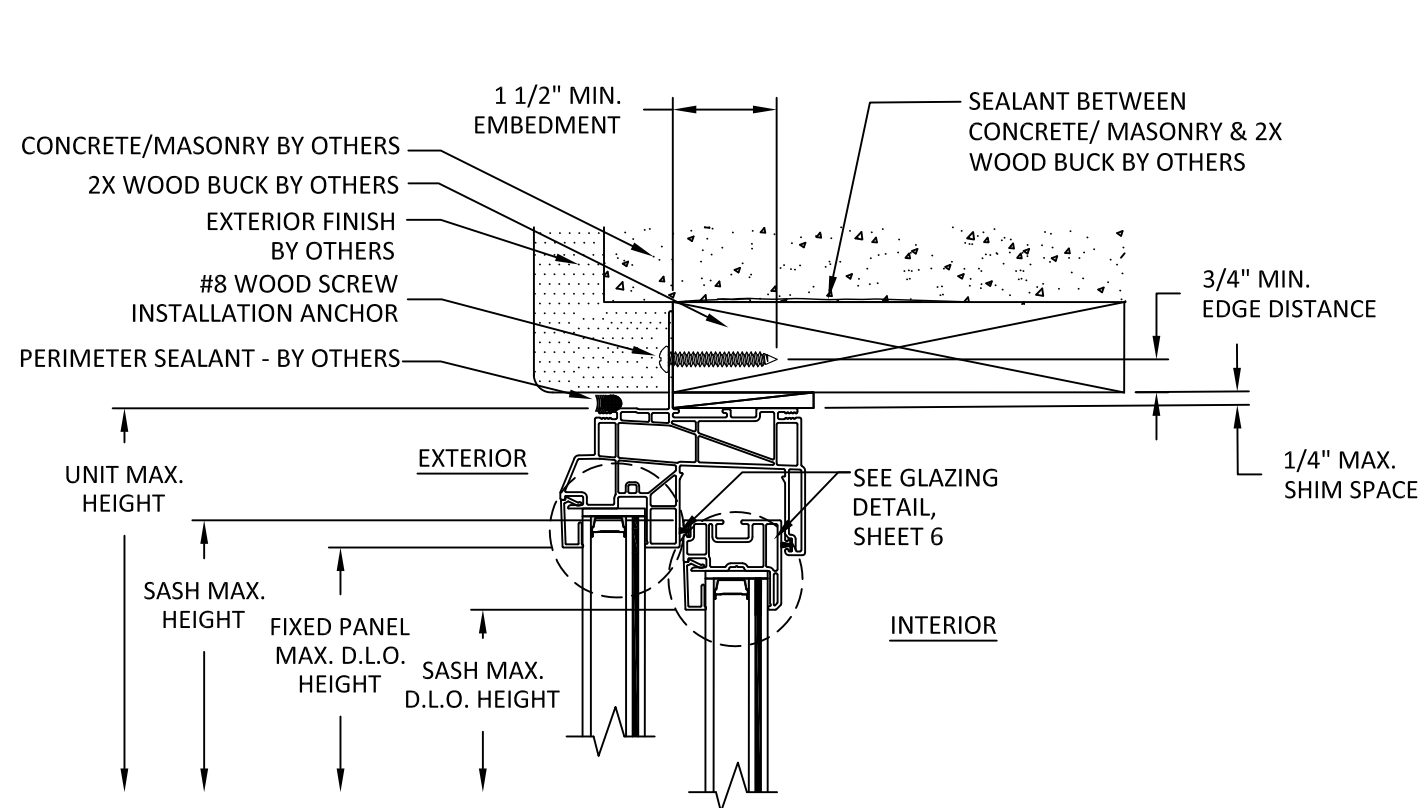
A 3 VERTICAL SECTION NAIL FIN INSTALLATION WOOD BUCK
