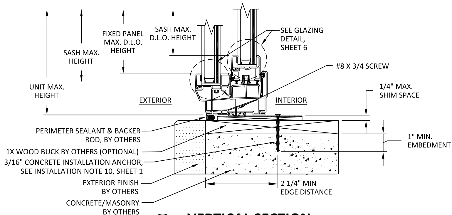
C 5 VERTICAL SECTION CLIP INSTALLATION CONCRETE/CMU
