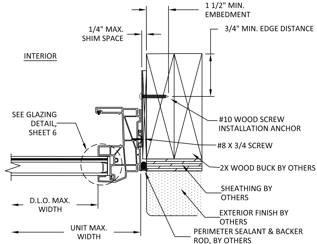
D 5 HORIZONTAL SECTION CLIP INSTALLATION WOOD SUBSTRATE
