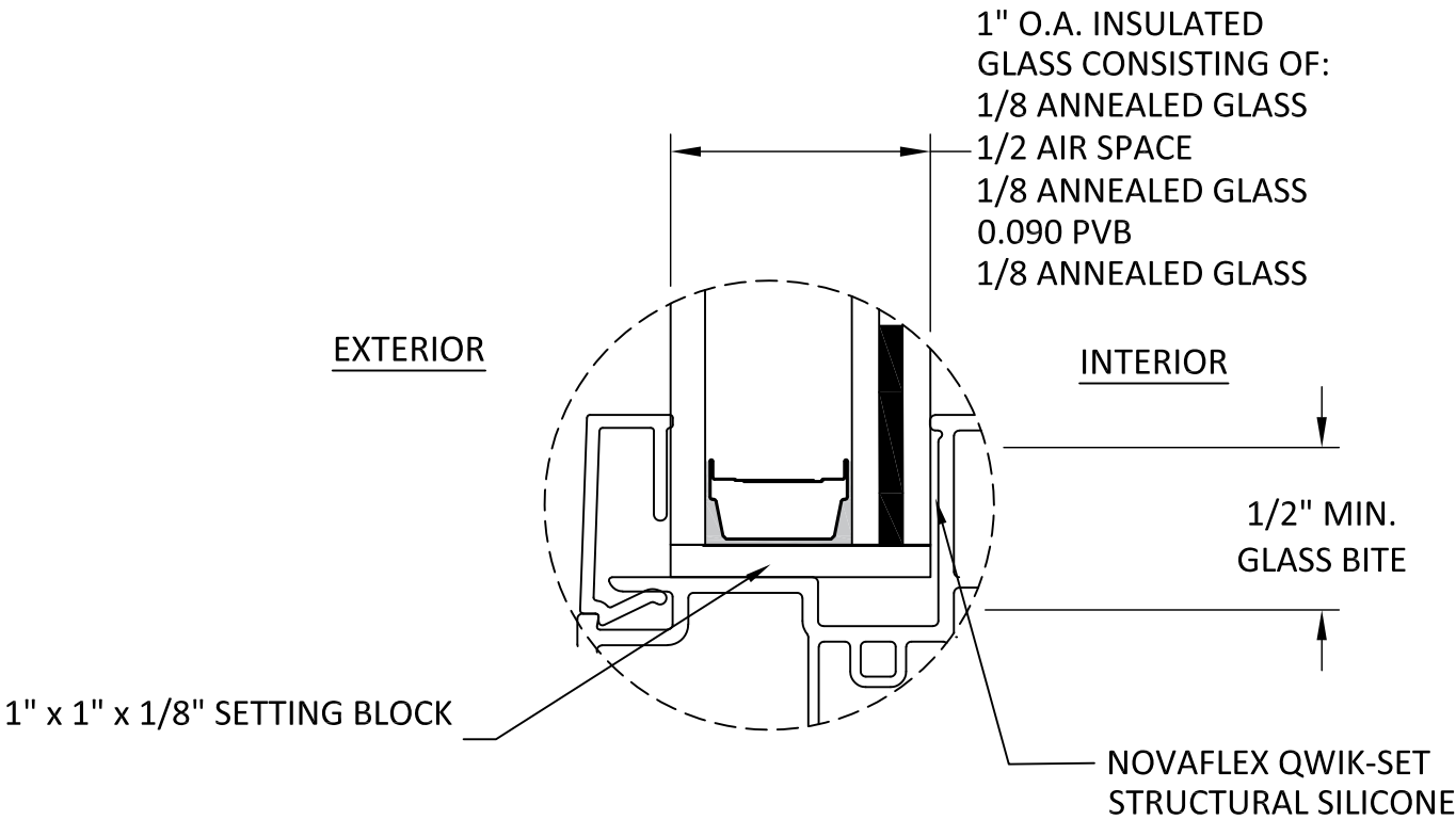
GLAZING DETAIL
