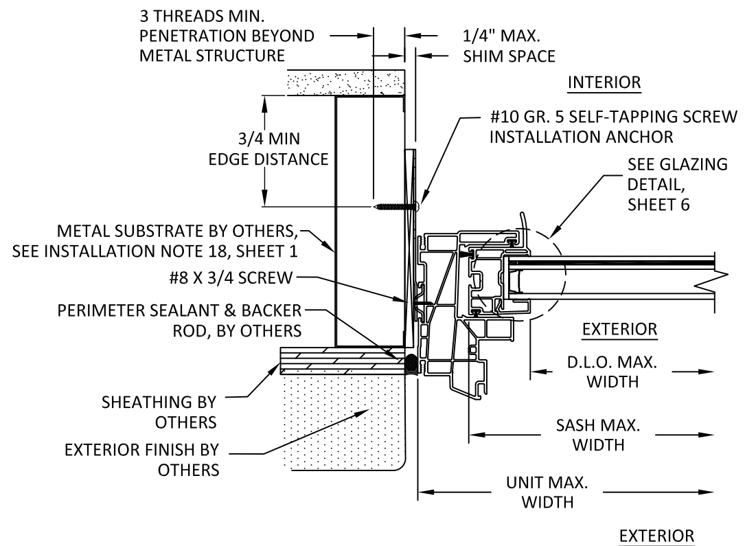
B 5 HORIZONTAL SECTION CLIP INSTALLATION METAL SUBSTRATE
